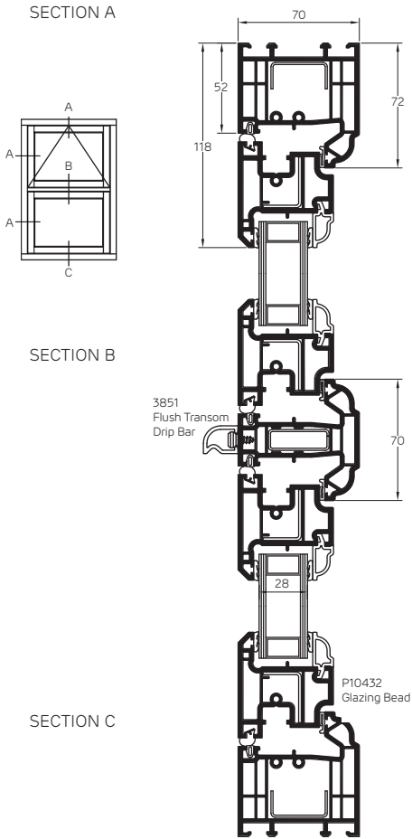
Flush70 72mm Outer Frame Large
