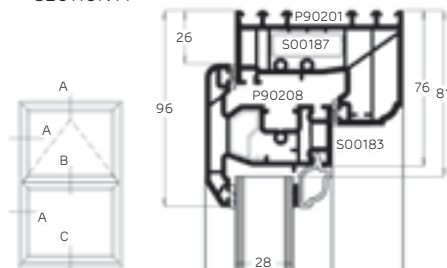
SECTION A
