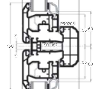
SECTION B
