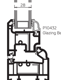
CLARITY 56mm Flush Outer Frame Slim
