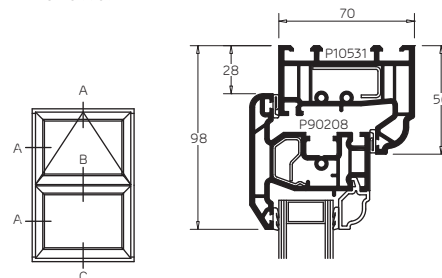
SECTION A
