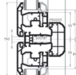
SECTION B
