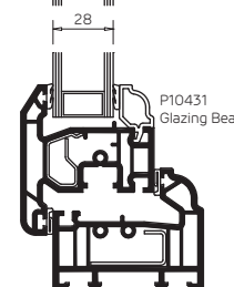
CLARITY 56mm Storm Outer Frame Slim
