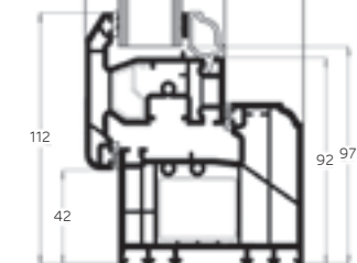
SECTION C
