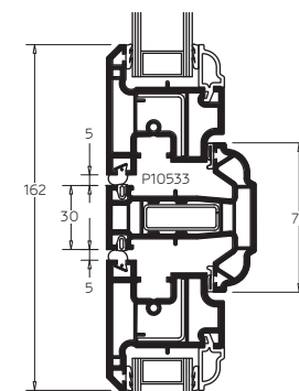
SECTION B
