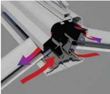
Ventilated roof ridge
